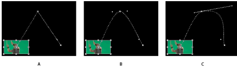
A Linear spatial keyframe B Auto Bezier interpolation C Continuous Bezier interpolation
