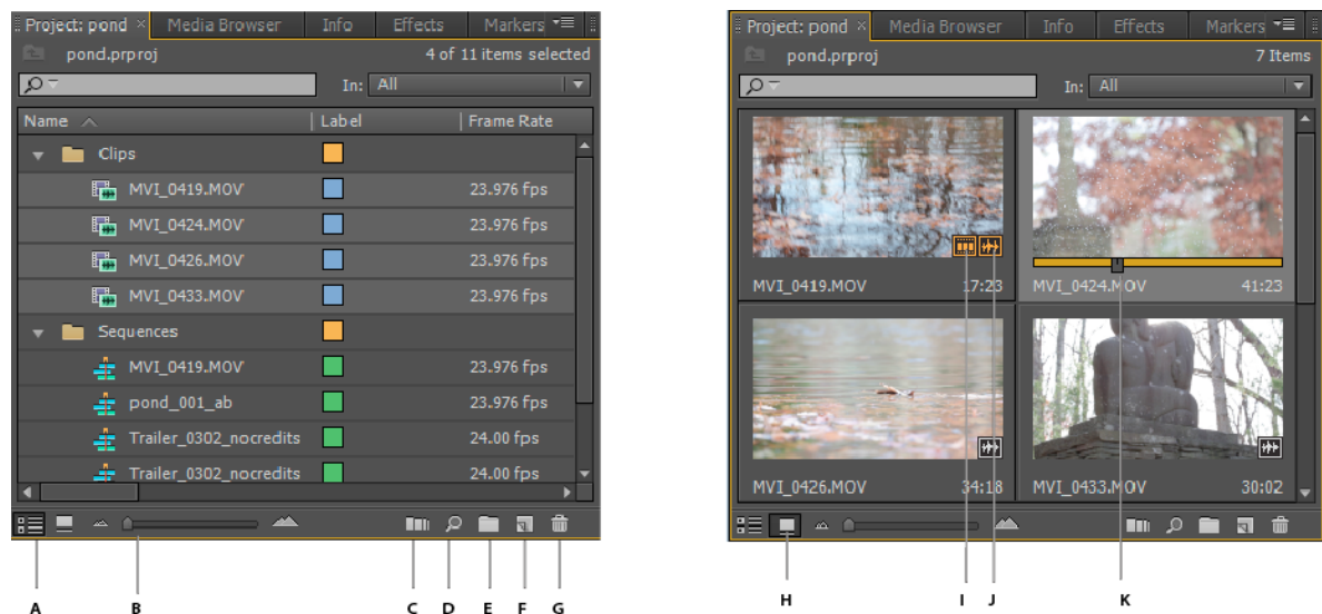
A List view B Zoom slider C Automate to sequence D Find E New Bin F New item G Clear H Icon view I Clip used in a sequence J Clip contains both audio and video K Playhead for scrubbing the thumbnail
