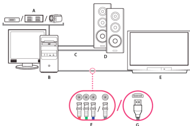
A Card reader, drive, or camcorder for P2, XDCAM HD, XDCAM EX, or AVCHD media B Computer and computer monitor C Audio cables running to speakers or amplifier D Speakers E TV monitor F BNC connectors for component or SDI video cables to TV monitor (alternative to "G") G HDMI connector for audio-video cable to TV monitor (alternative to "F")
