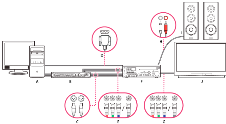
A Computer and computer monitor B (Optional) A/V breakout box C XLR jacks and plugs for L & R audio D RS232/422 port and connector E BNC jacks and plugs for Y/Pb/Pr component video, BNC jack, and plug for SDI video F HD/SD VTR G BNC jacks and plugs for Y/Pb/Pr component video, BNC jack, and plug for SDI video H RCA jacks and plugs for L (white) & R (red) audio I Speakers J Television monitor
