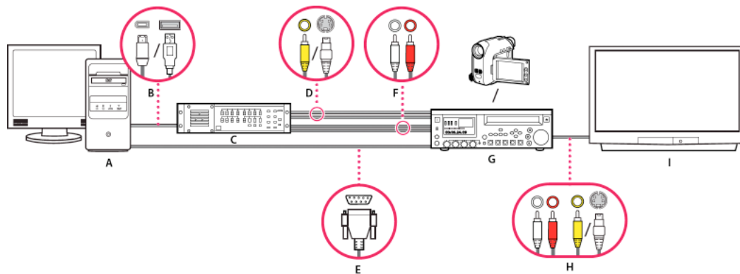
A Computer and computer monitor B Ports and connectors for FireWire, USB 2.0 C A/D converter D Jacks and plugs for RCA composite video, S-Video (y/c) E RS 232/422 port and connector F RCA jacks and plugs for L (white) and R (red) audio G Analog camcorder, analog VTR H RCA jacks and plugs for L (white) audio, R (red) audio, and composite video (yellow); jack and plug for S-Video (y/c) I Television monitor
