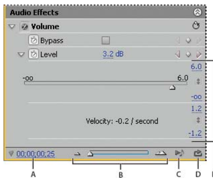
A Current time B Zoom controls C Play Only The Audio For This Clip D Toggle Looping Audio Playback E Effect values
