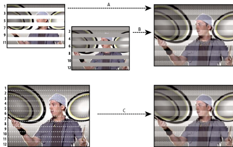
A For interlaced video, entire upper field (odd-numbered lines) is drawn to screen first, from top to bottom, in one pass. B Next, entire lower field (even-numbered lines) is drawn to screen, from top to bottom, in one pass. C For noninterlaced video, entire frame (all lines in counting order) is drawn to screen, from top to bottom, in one pass.
